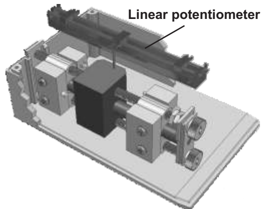
Limit switch version 2P (not MR6) for applications with defined stops in both directions, protected by 2 safety switches. Additional potentiometer signal for positioning.
