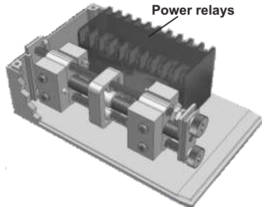
Limit switch version 1 (not MR6) for applications with defined stops in both directions, protected by 2 safety switches, with integrated power relays.
